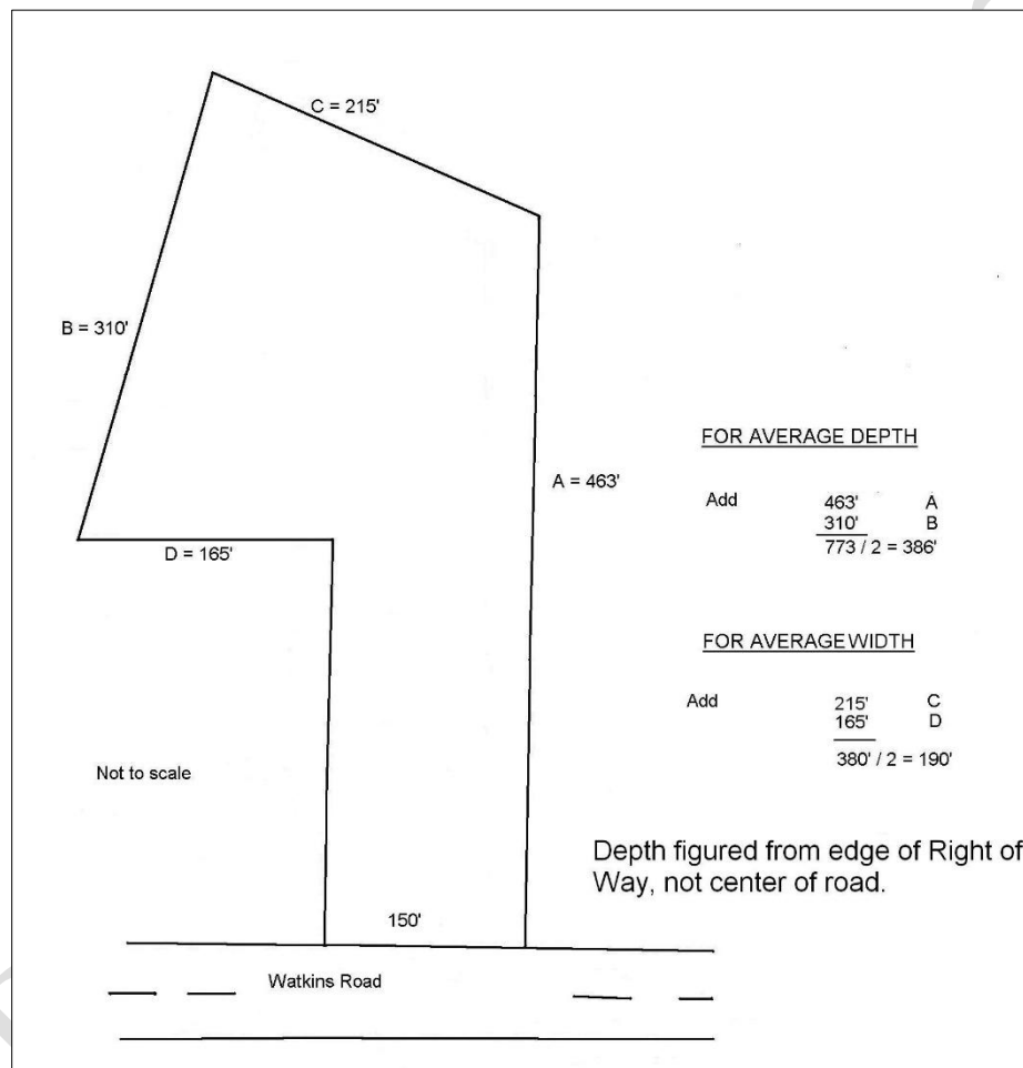
Diagram 3 (Existing Method).
