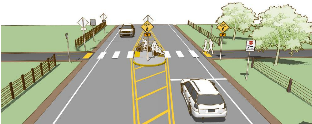
Exhibit 4.8 – Option 3 Crossing Application (image credit: Small Town and Rural Multimodal Networks, FHWA)
