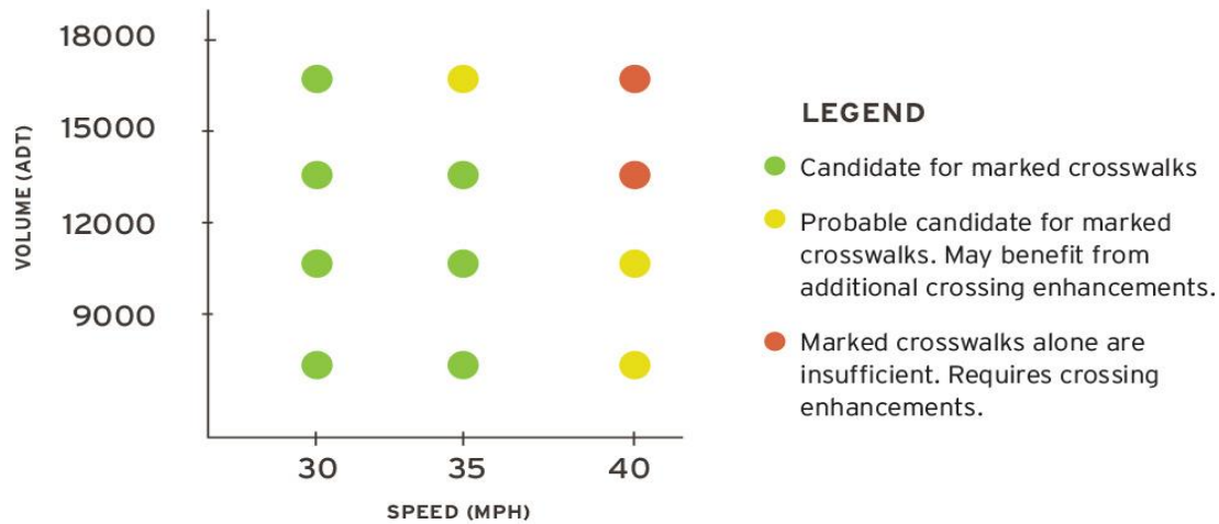
Exhibit 4.5 – Crossing Enhancement Recommendations based on Volume and Speed (image credit: Small Town and Rural Multimodal Networks, FHWA)
