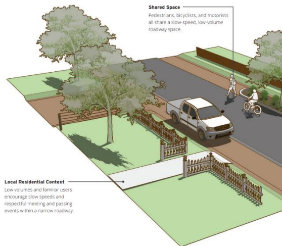
Exhibit 4.3 – Shared or Yield Roadway (image credit: Small Town and Rural Multimodal Networks, FHWA)
