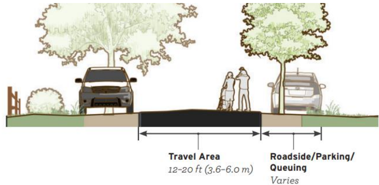
Exhibit 4.3 – Shared or Yield Roadway (image credit: Small Town and Rural Multimodal Networks, FHWA)
