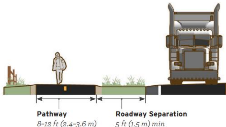
Exhibit 4.2 – Trail Typical Section adjacent to roadway (image credit: Small Town and Rural Multimodal Networks, FHWA)
