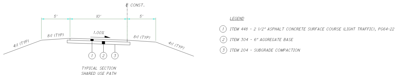
Exhibit 4.1 – Trail Typical Section on Abandoned Rail Bed
