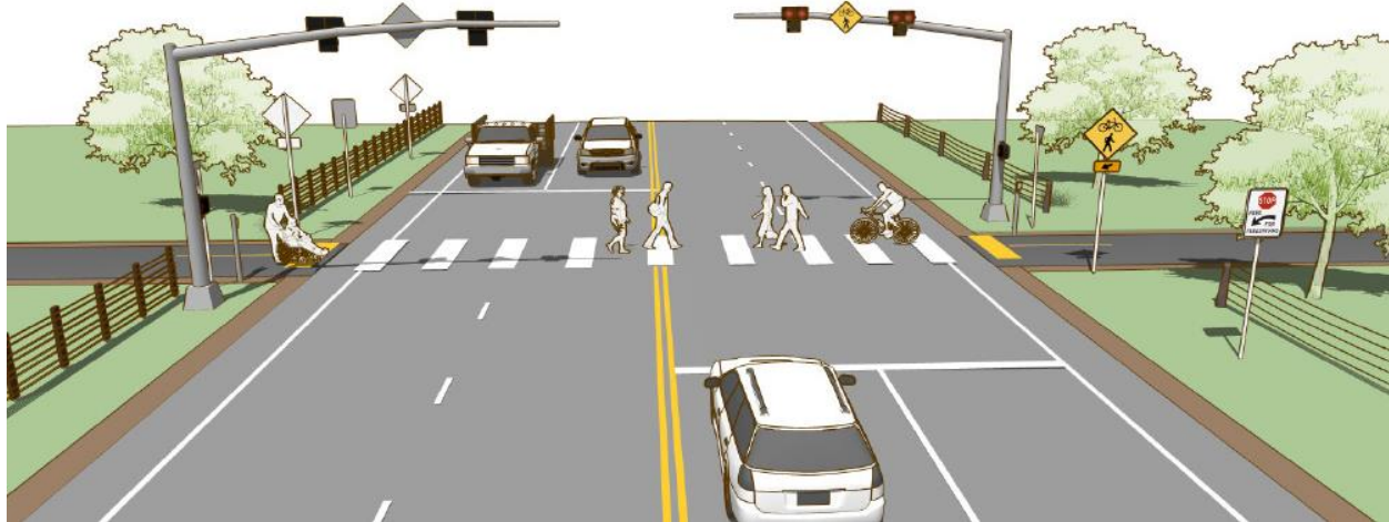
Exhibit 4.9 – Option 4 Crossing Application (image credit: Small Town and Rural Multimodal Networks, FHWA)
