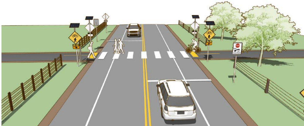
Exhibit 4.7 – Option 2 Crossing Application (image credit: Small Town and Rural Multimodal Networks, FHWA)
