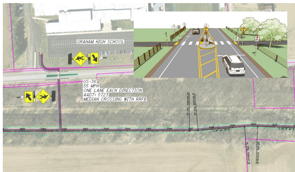
Exhibit 4.13 – Potential Trail Connection to Graham High School
